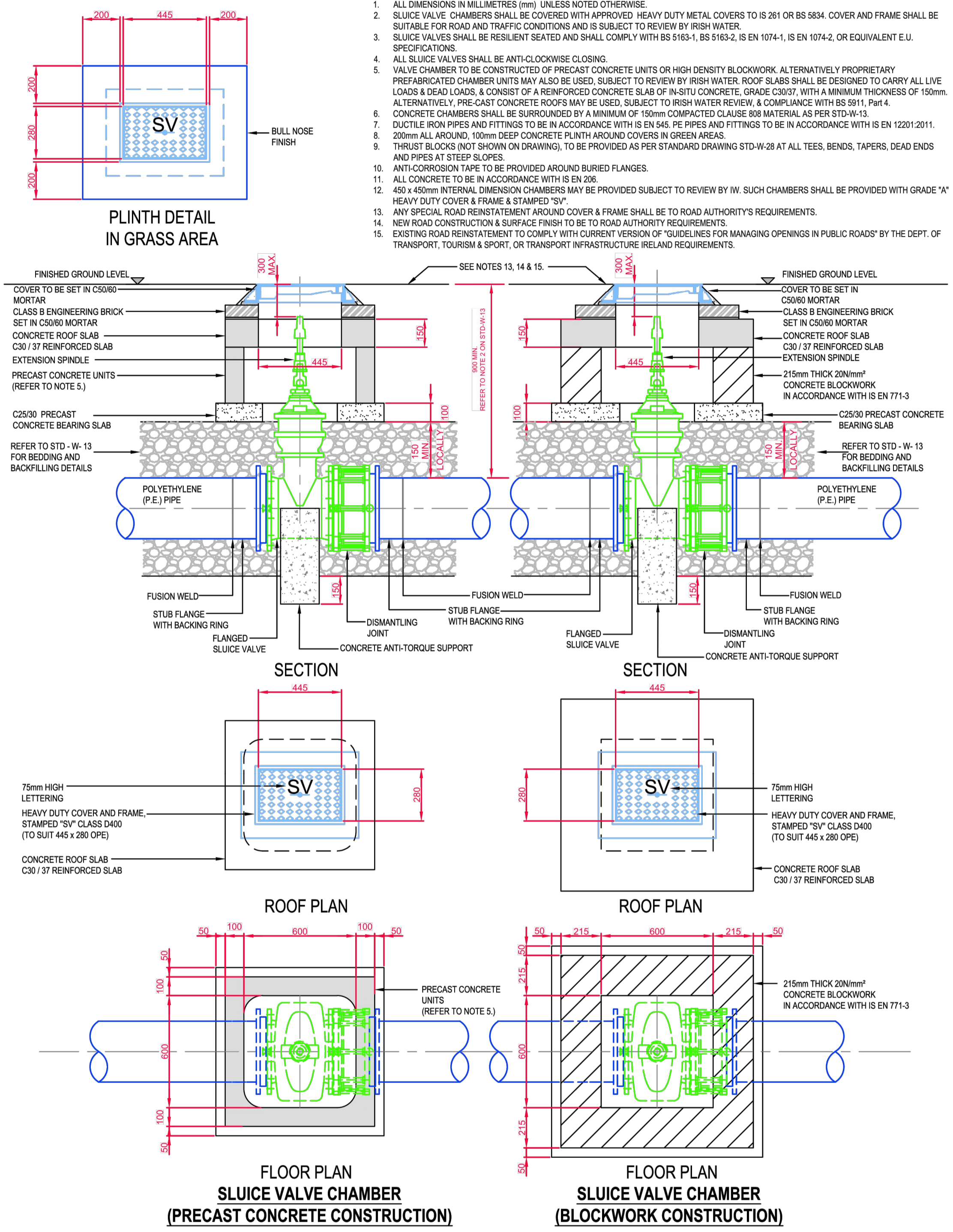
SLUISE VALVE FOR POLYETHYLENE (P.E.) PIPE (<350mm DIA.) (STD-W-15)
