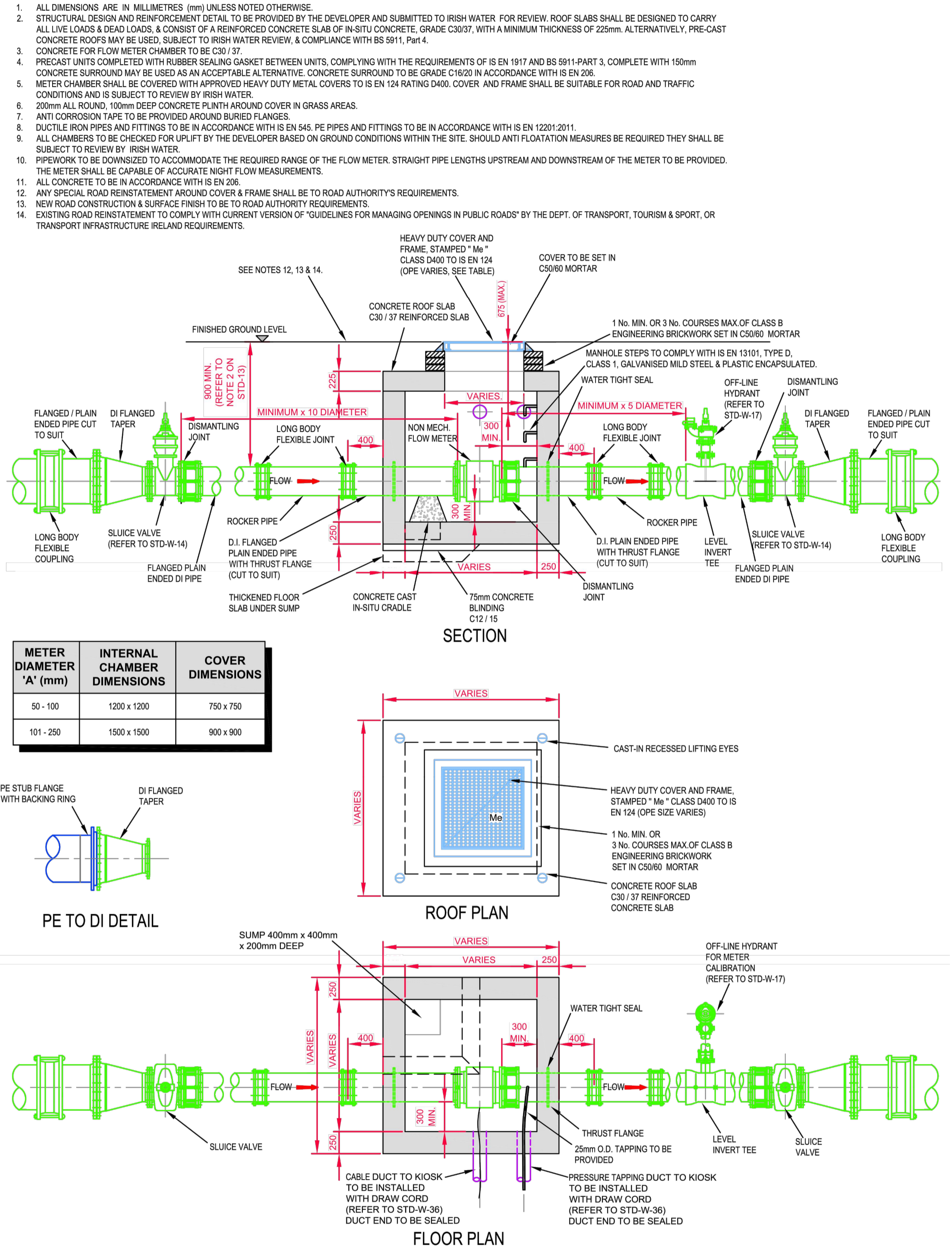
NON-MECH. METER CHAMBER (40-250mm DIA.) (STD-W-26)
